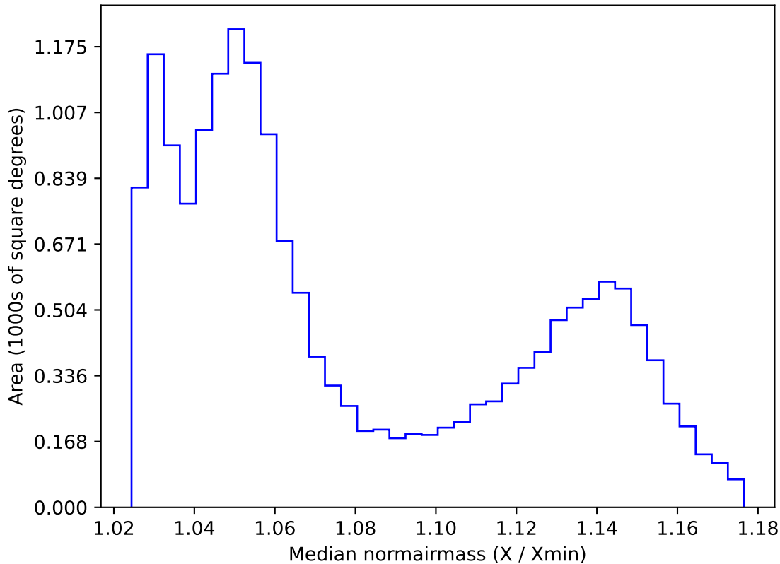
ddf_acor_sf10_lsf30_lsr50_v3.4_10yrs WFD all bands: Median normairmass
