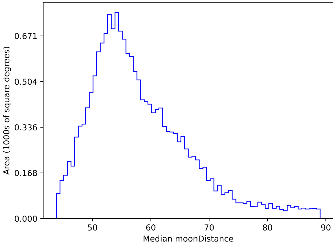
ddf_acor_sf10_lsf30_lsr50_v3.4_10yrs WFD y band: Median moonDistance
