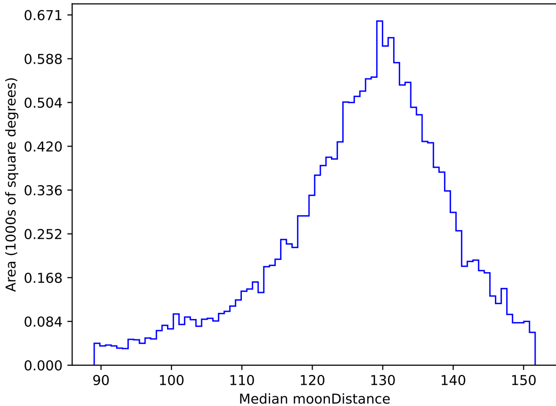
ddf_acor_sf10_ls30_lsr50_v3.4_10yrs WFD u band: Median moonDistance
