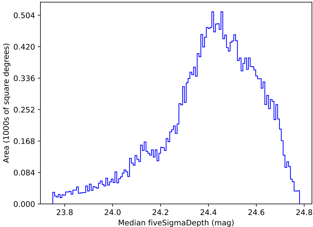
ddf_acor_sf10_lsf30_lsr50_v3.4_10yrs All sky g band: Median fiveSigmaDepth
