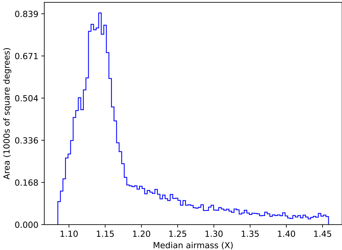
ddf_acor_sf10_lsf30_lsr50_v3.4_10yrs WFD all bands: Median airmass
