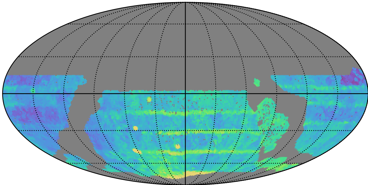
ddf_acor_sf10_lsf30_lsr50_v3.4_10yrs WFD all bands: Median Season Length
