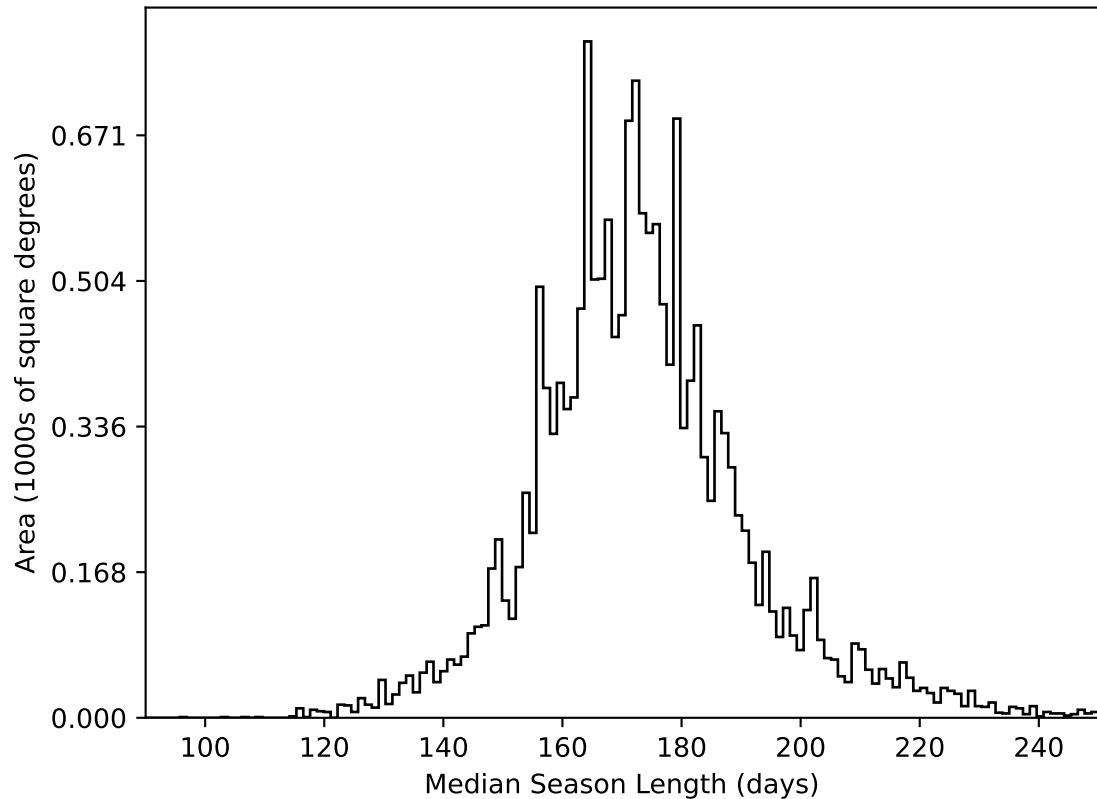
ddf_acor_sf10_lsf30_lsr50_v3.4_10yrs WFD all bands: Median Season Length
