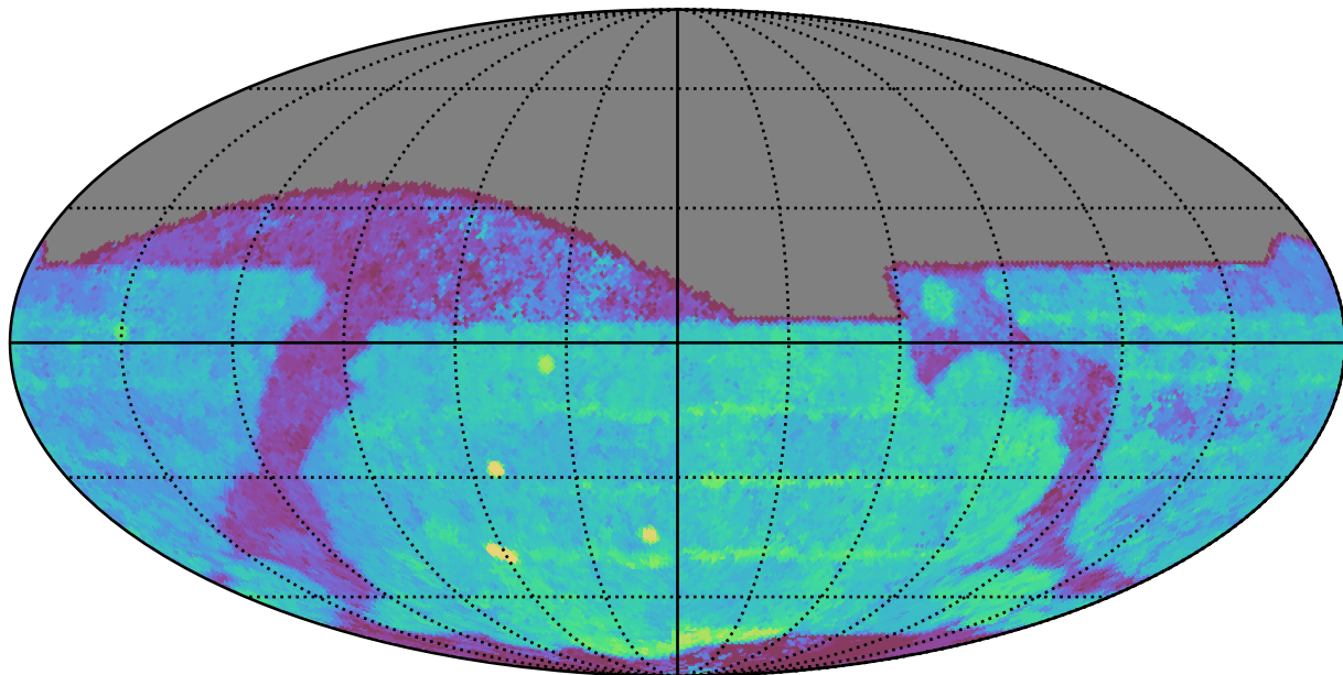
ddf_acor_sf10_lsf30_lsr50_v3.4_10yrs All sky z band: Median Season Length
