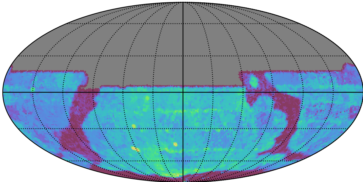
ddf_acor_sf10_lsf30_lsr50_v3.4_10yrs All sky y band: Median Season Length
