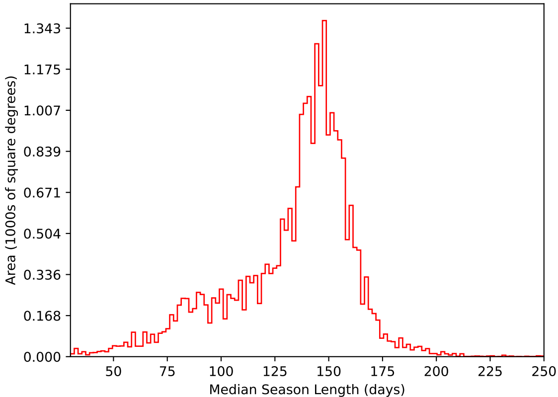
ddf_acor_sf10_lsf30_lsr50_v3.4_10yrs All sky i band: Median Season Length
