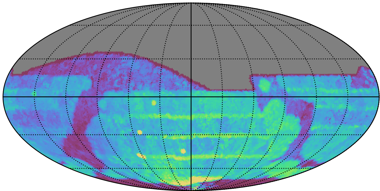
ddf_acor_sf10_lsf30_lsr50_v3.4_10yrs All sky all bands: Median Season Length
