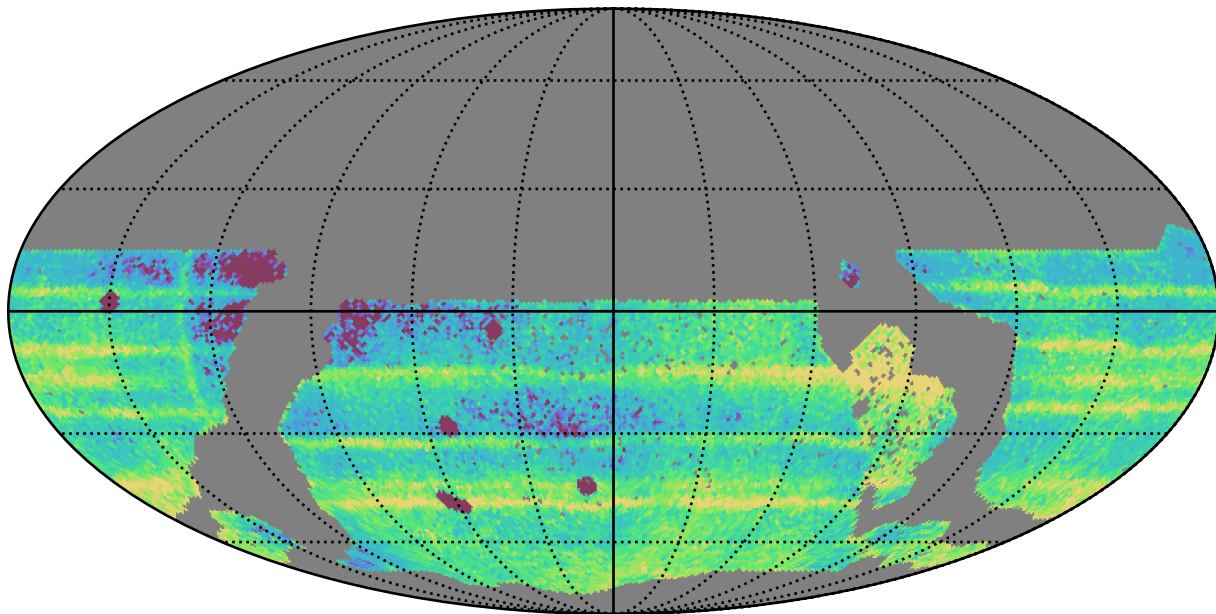
ddf_acor_sf10_lsf30_lsr50_v3.4_10yrs WFD: Median Intra-Night Gap
