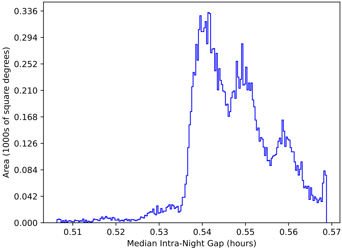
ddf_acor_sf10_ls30_lsr50_v3.4_10yrs WFD: Median Intra-Night Gap
