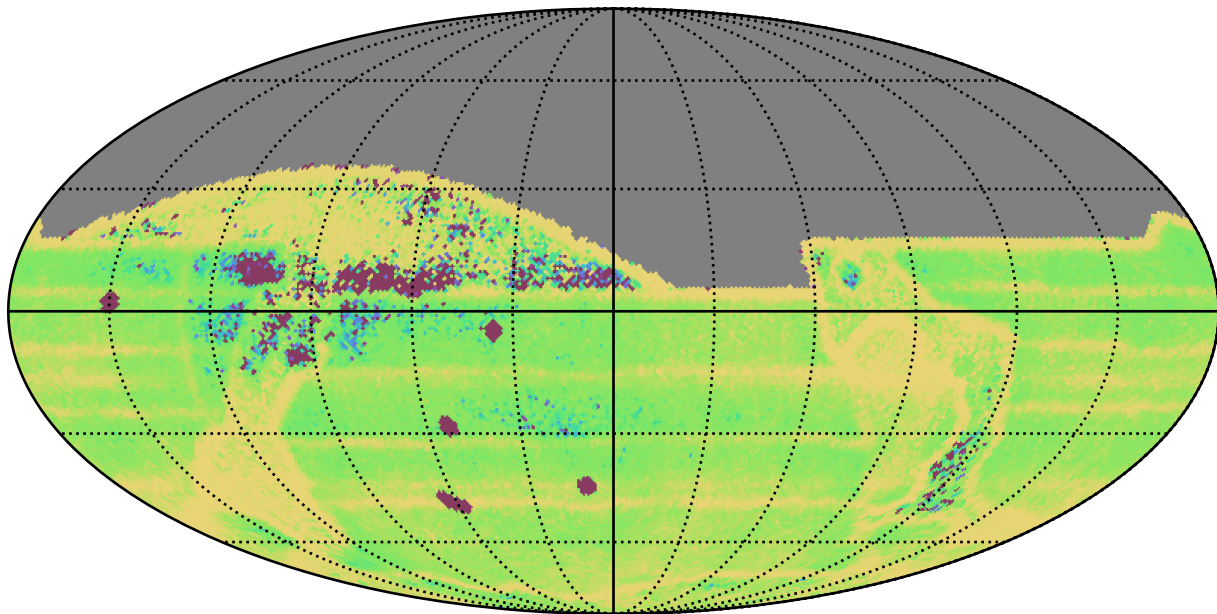
ddf_acor_sf10_lsf30_lsr50_v3.4_10yrs All sky: Median Intra-Night Gap
