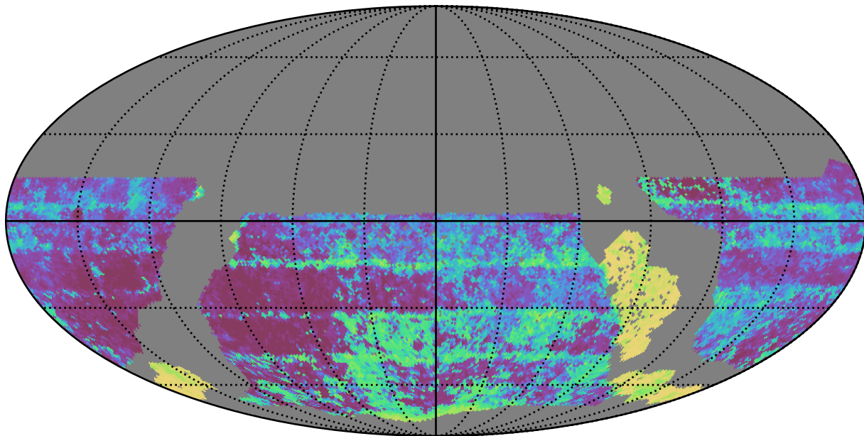
ddf_acor_sf10_lsf30_lsr50_v3.4_10yrs WFD y band: Median Inter-Night Gap
