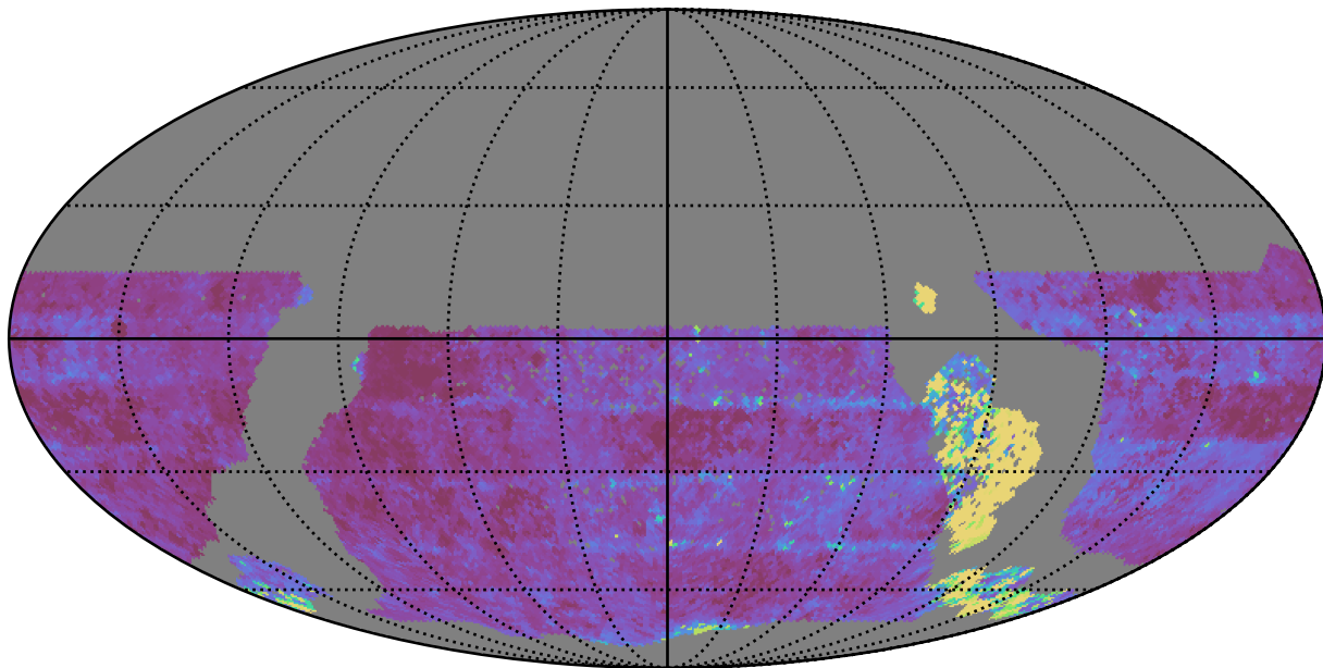
ddf_acor_sf10_lsf30_lsr50_v3.4_10yrs WFD u band: Median Inter-Night Gap
