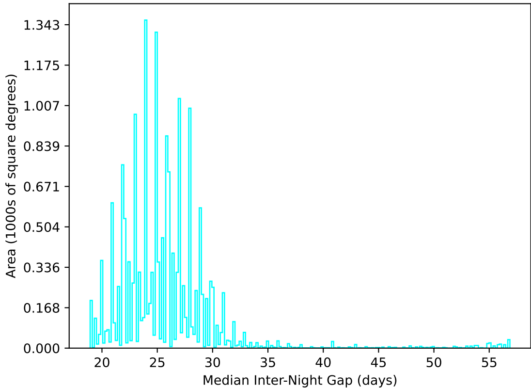
ddf_acor_sf10_lsf30_lsr50_v3.4_10yrs WFD u band: Median Inter-Night Gap
