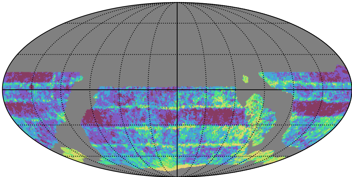
ddf_acor_sf10_lsf30_lsr50_v3.4_10yrs WFD r band: Median Inter-Night Gap
