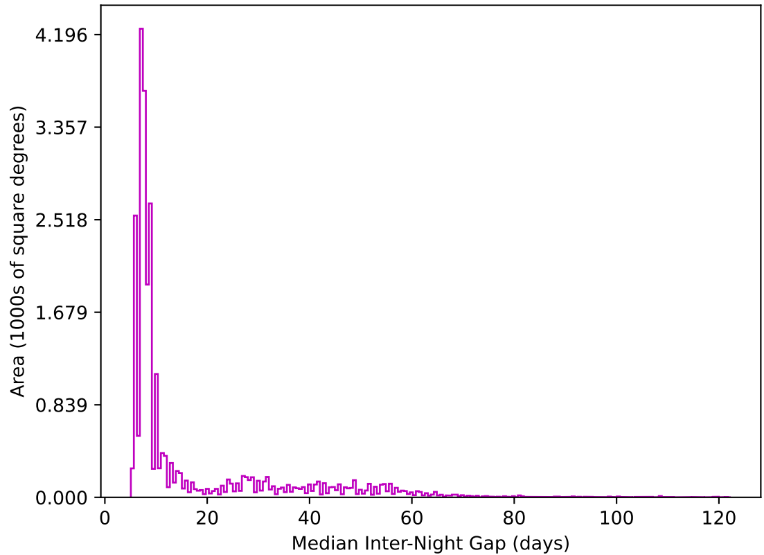
ddf_acor_sf10_lsf30_lsr50_v3.4_10yrs All sky z band: Median Inter-Night Gap
