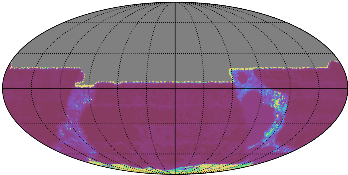
ddf_acor_sf10_lsf30_lsr50_v3.4_10yrs All sky y band: Median Inter-Night Gap
