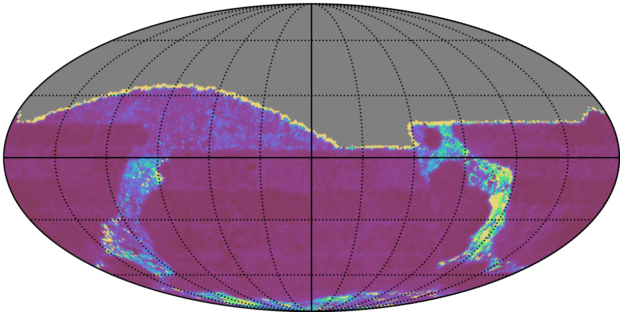
ddf_acor_sf10_lsf30_lsr50_v3.4_10yrs All sky g band: Median Inter-Night Gap
