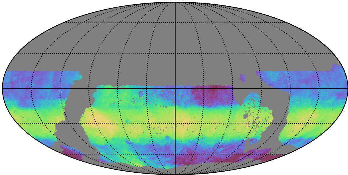
ddf_acor_sf10_lsf30_lsr50_v3.4_10yrs WFD z band: Median HA
