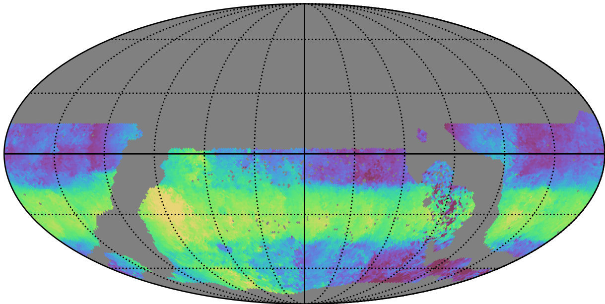
ddf_acor_sf10_lsf30_lsr50_v3.4_10yrs WFD u band: Median HA
