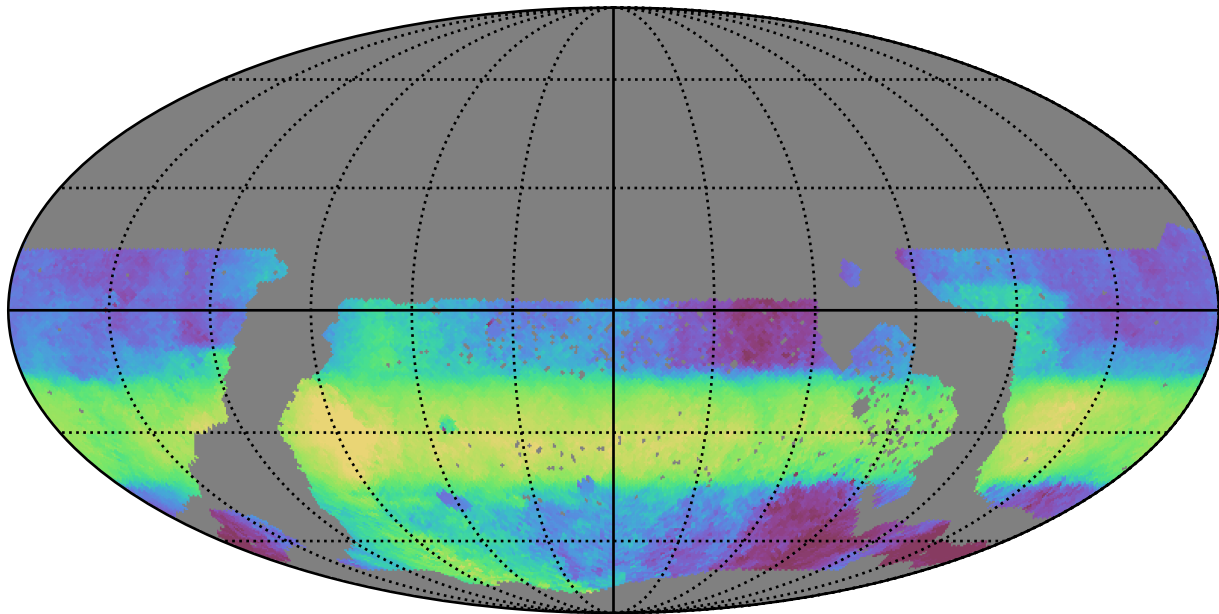
ddf_acor_sf10_lsf30_lsr50_v3.4_10yrs WFD r band: Median HA
