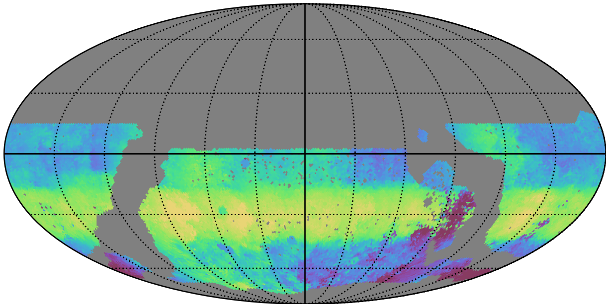
ddf_acor_sf10_lsf30_lsr50_v3.4_10yrs WFD g band: Median HA
