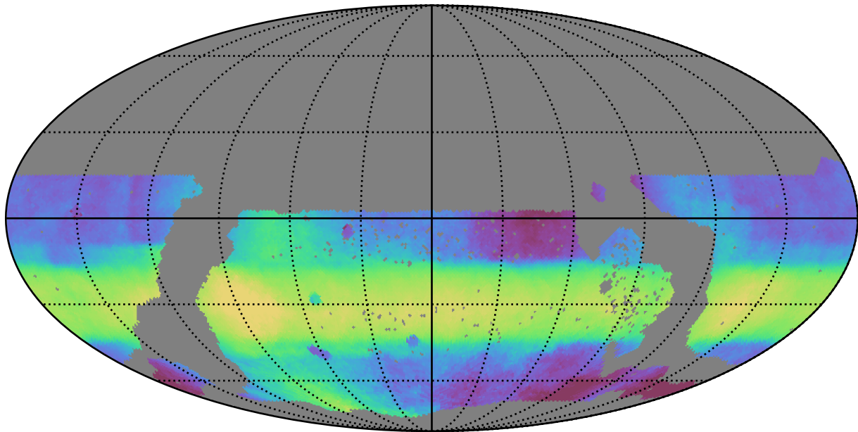
ddf_acor_sf10_lsf30_lsr50_v3.4_10yrs WFD all bands: Median HA
