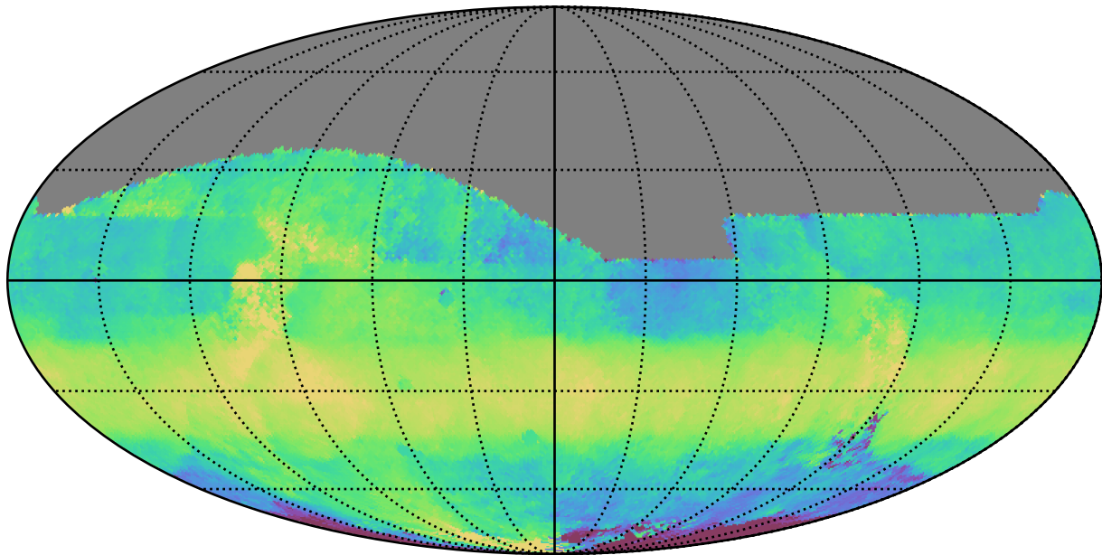
ddf_acor_sf10_lsf30_lsr50_v3.4_10yrs All sky z band: Median HA
