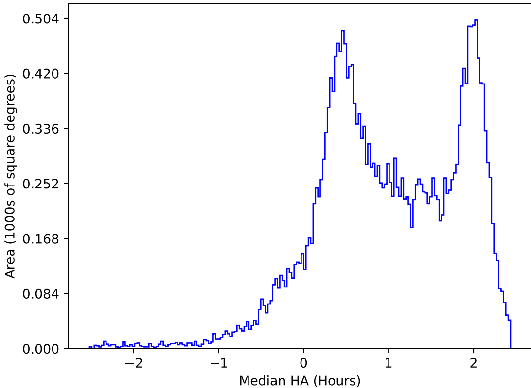
ddf_acor_sf10_lsf30_lsr50_v3.4_10yrs All sky z band: Median HA
