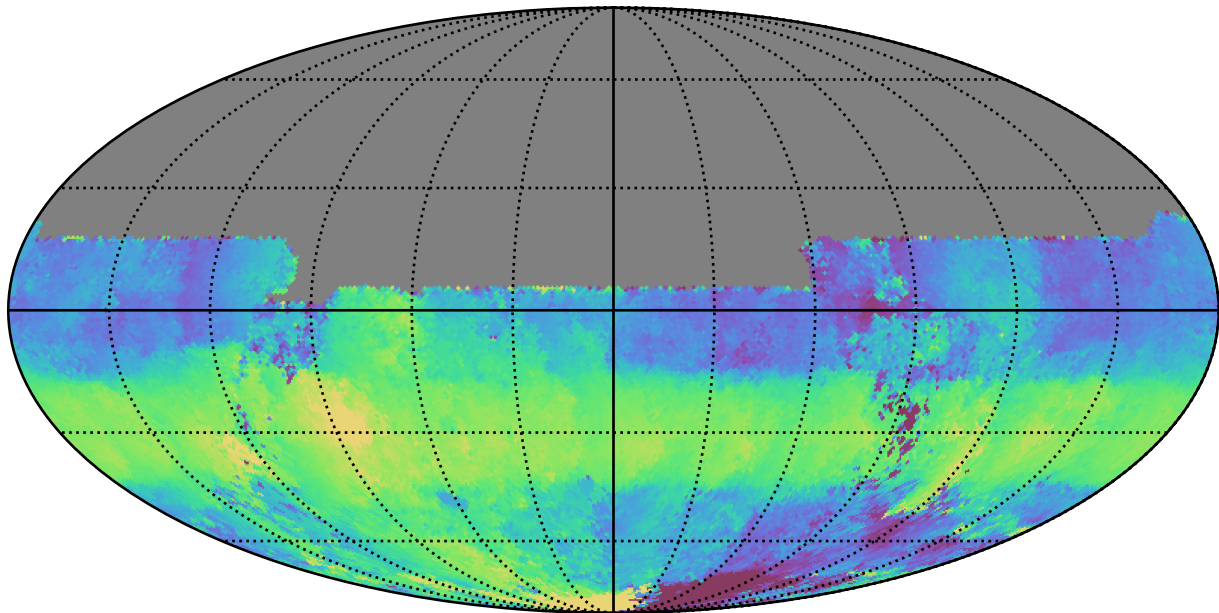
ddf_acor_sf10_lsf30_lsr50_v3.4_10yrs All sky u band: Median HA
