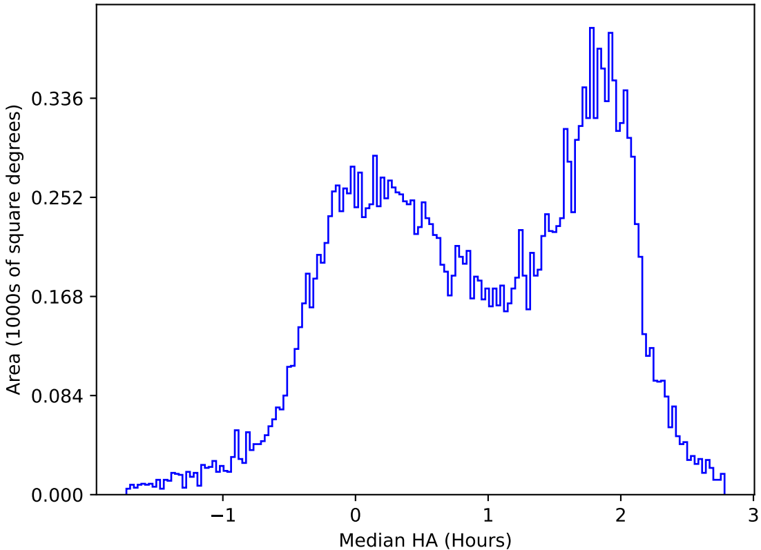
ddf_acor_sf10_ls30_lsr50_v3.4_10yrs All sky u band: Median HA
