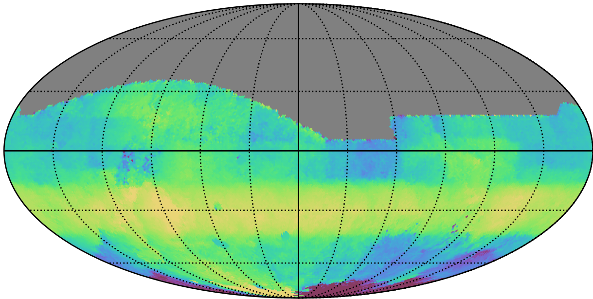
ddf_acor_sf10_lsf30_lsr50_v3.4_10yrs All sky r band: Median HA
