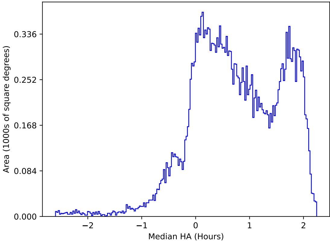
ddf_acor_sf10_lsf30_lsr50_v3.4_10yrs All sky r band: Median HA
