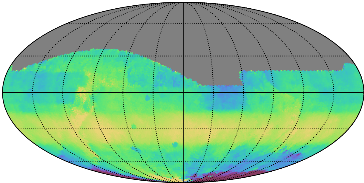
ddf_acor_sf10_lsf30_lsr50_v3.4_10yrs All sky i band: Median HA
