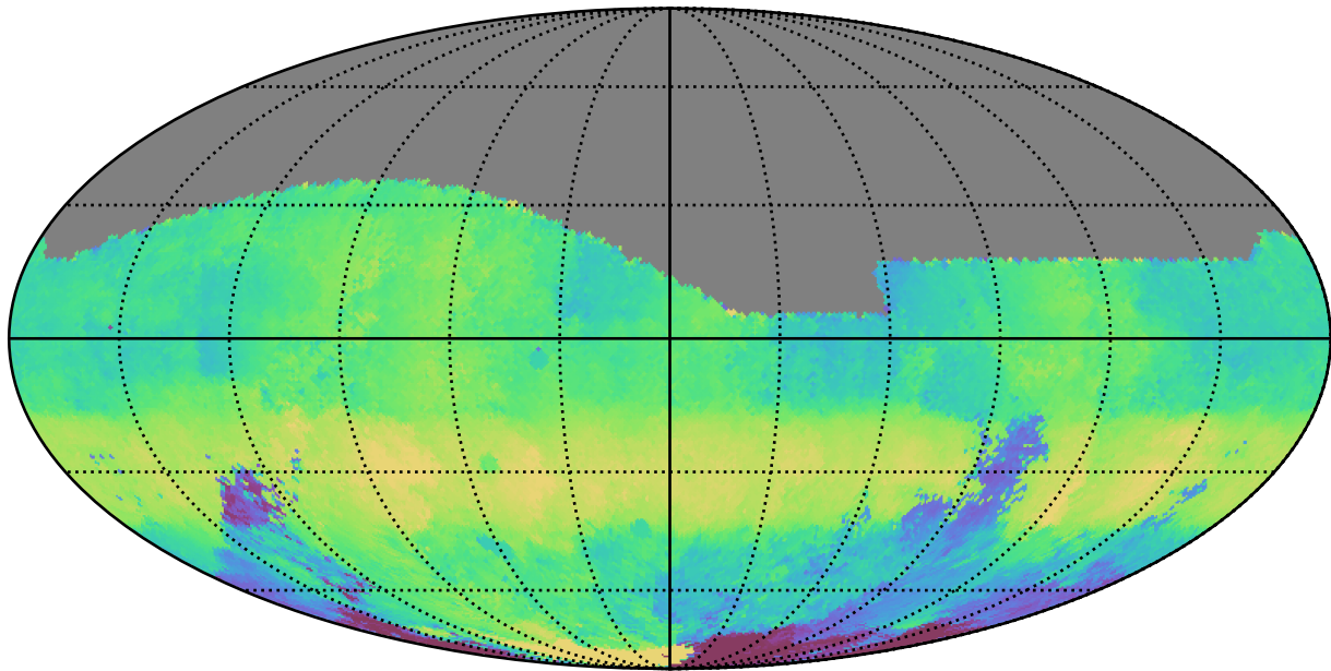
ddf_acor_sf10_lsf30_lsr50_v3.4_10yrs All sky g band: Median HA
