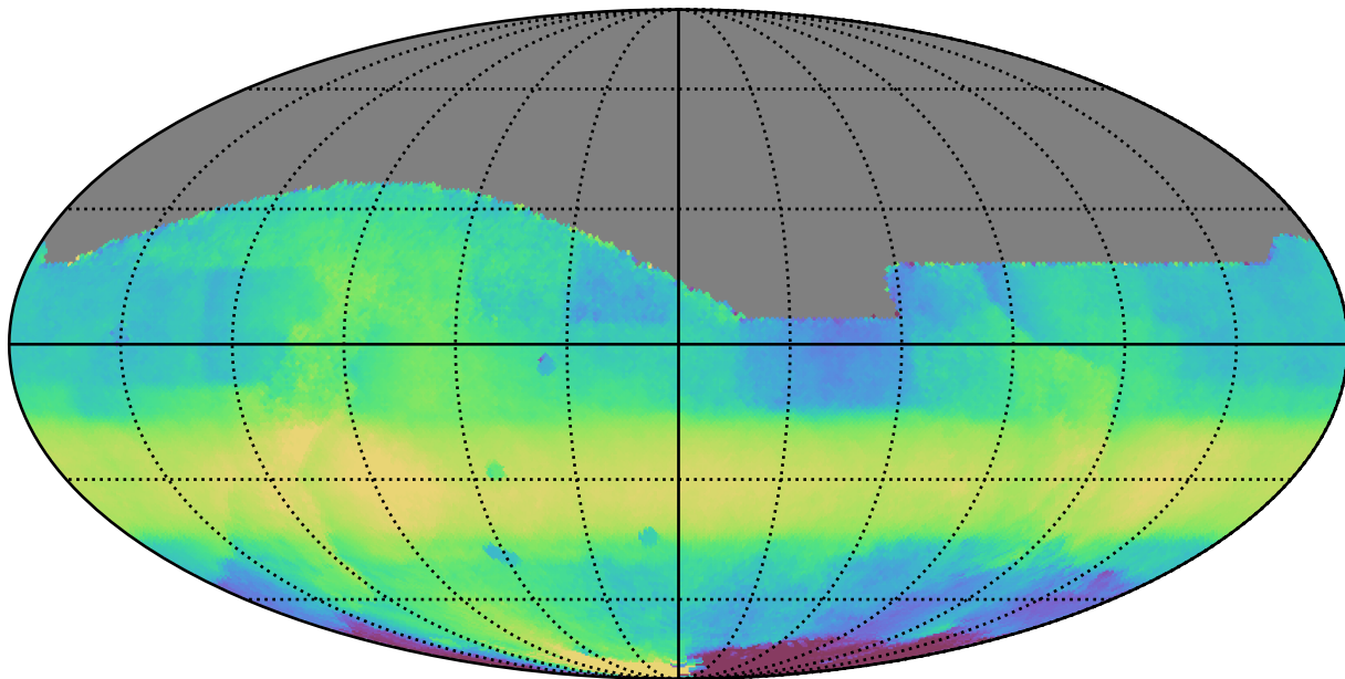
ddf_acor_sf10_lsf30_lsr50_v3.4_10yrs All sky all bands: Median HA
