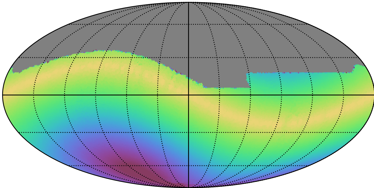
ddf_acor_sf10_lsf30_lsr50_v3.4_10yrs All sky i band: Max solarElong
