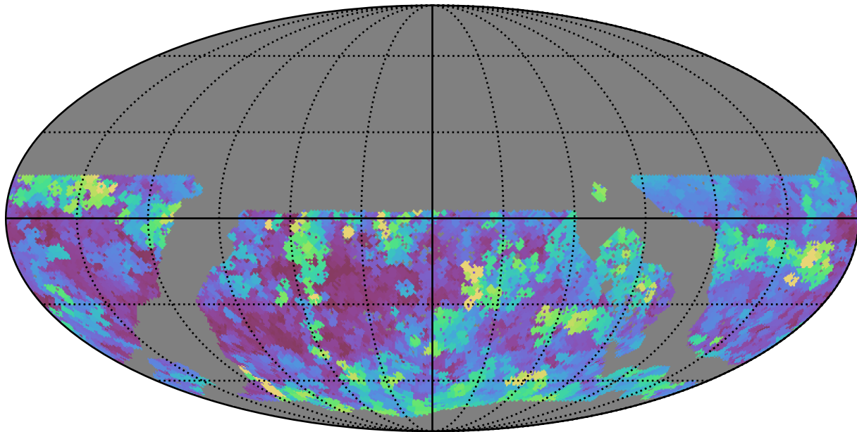
ddf_acor_sf10_lsf30_lsr50_v3.4_10yrs WFD g band: Max seeingEff
