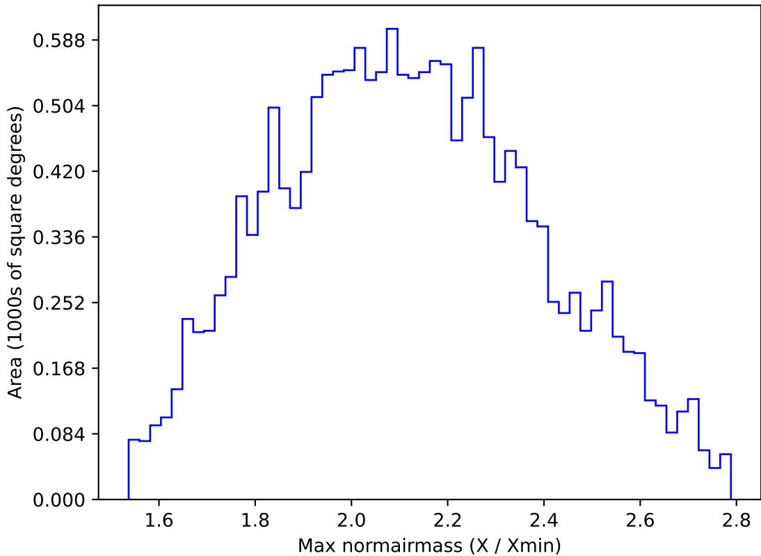
ddf_acor_sf10_lsf30_lsr50_v3.4_10yrs WFD y band: Max normairmass
