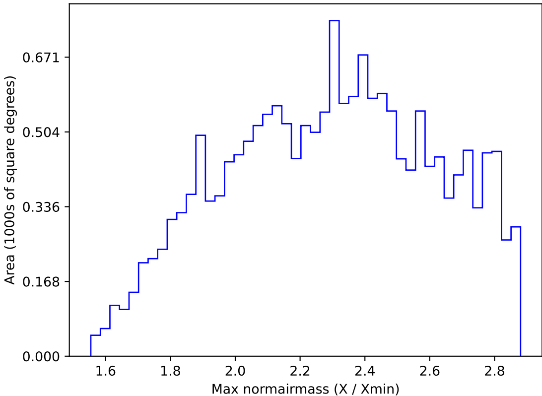
ddf_acor_sf10_lsf30_lsr50_v3.4_10yrs WFD i band: Max normairmass
