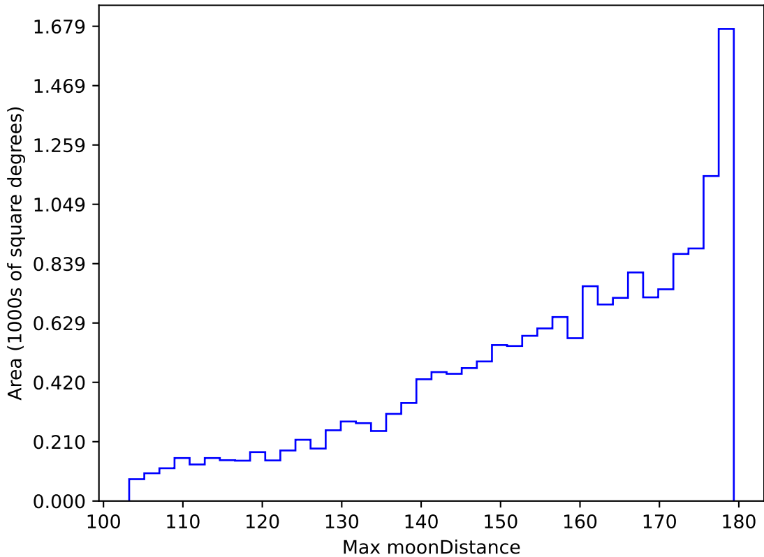
ddf_acor_sf10_lsf30_lsr50_v3.4_10yrs WFD r band: Max moonDistance
