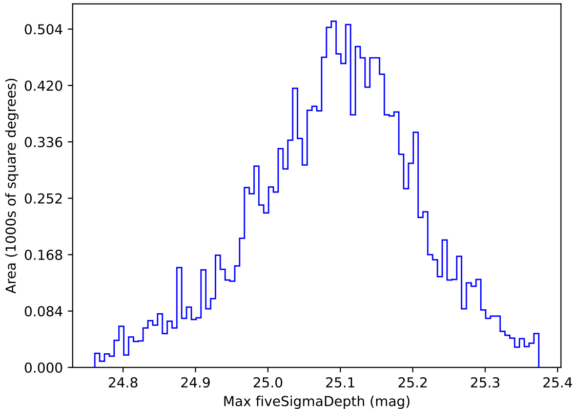
ddf_acor_sf10_lsf30_lsr50_v3.4_10yrs WFD all bands: Max fiveSigmaDepth
