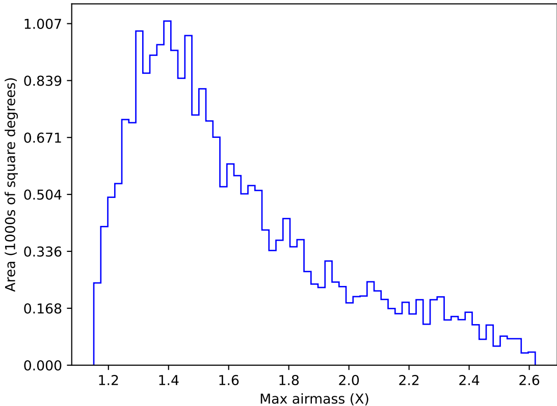
ddf_acor_sf10_lsf30_lsr50_v3.4_10yrs Yr 1 y band: Max airmass
