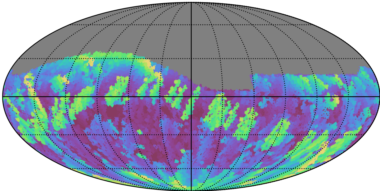
ddf_acor_sf10_lsf30_lsr50_v3.4_10yrs Yr 1 r band: Max airmass
