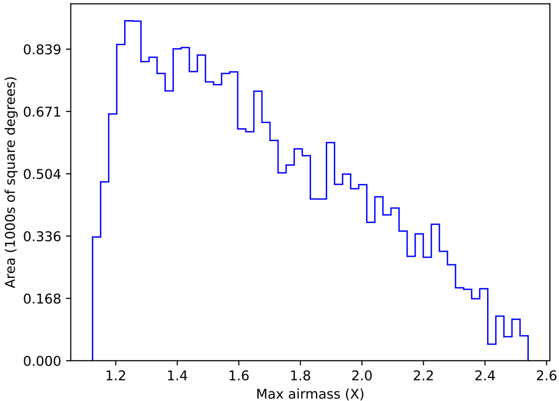
ddf_acor_sf10_lsf30_lsr50_v3.4_10yrs Yr 1 g band: Max airmass
