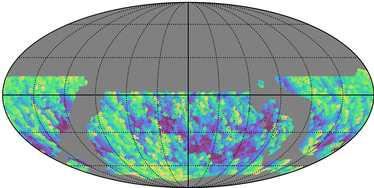
ddf_acor_sf10_lsf30_lsr50_v3.4_10yrs WFD y band: Max airmass
