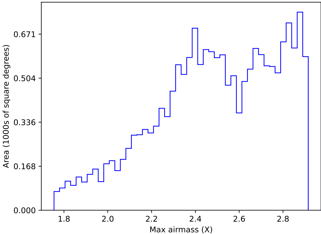
ddf_acor_sf10_lsf30_lsr50_v3.4_10yrs WFD i band: Max airmass
