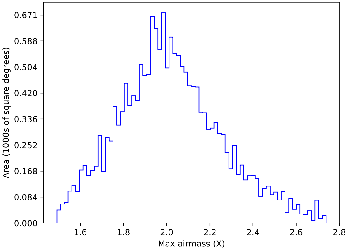
ddf_acor_sf10_ls30_lsr50_v3.4_10yrs WFD g band: Max airmass
