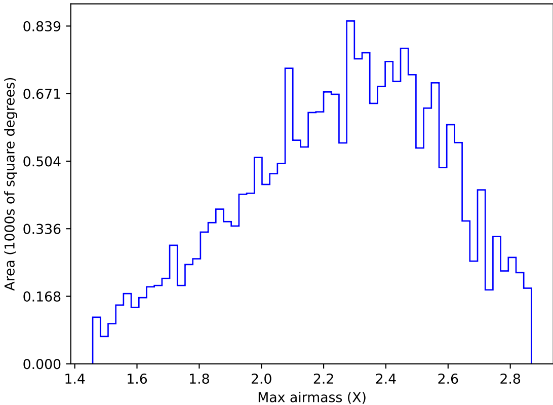
ddf_acor_sf10_lsf30_lsr50_v3.4_10yrs All sky y band: Max airmass
