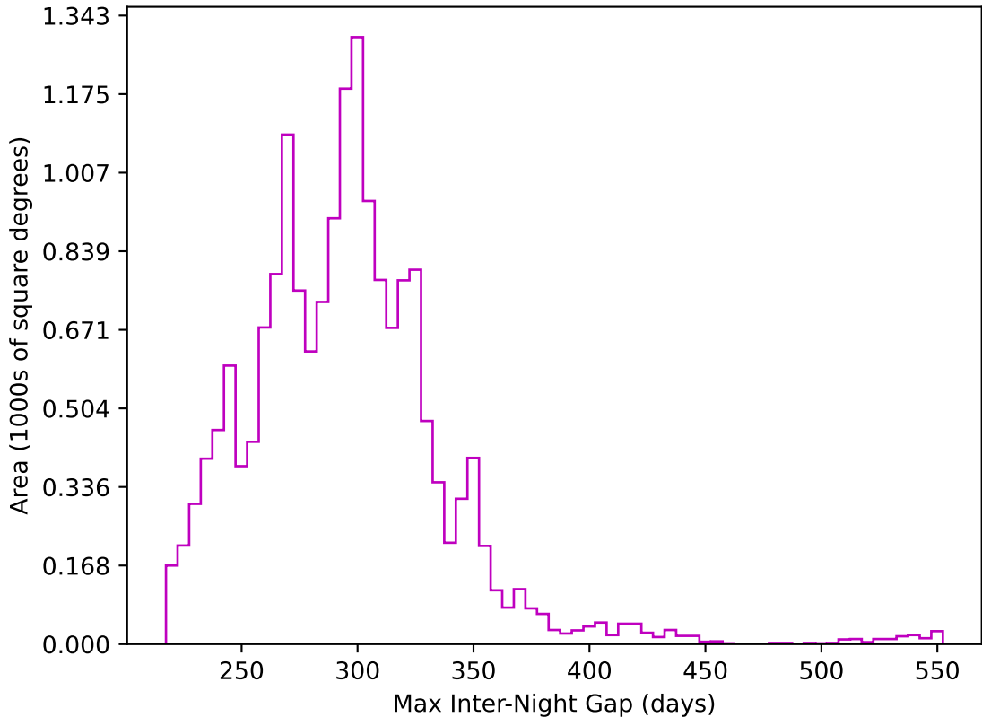
ddf_acor_sf10_lsf30_lsr50_v3.4_10yrs WFD z band: Max Inter-Night Gap
