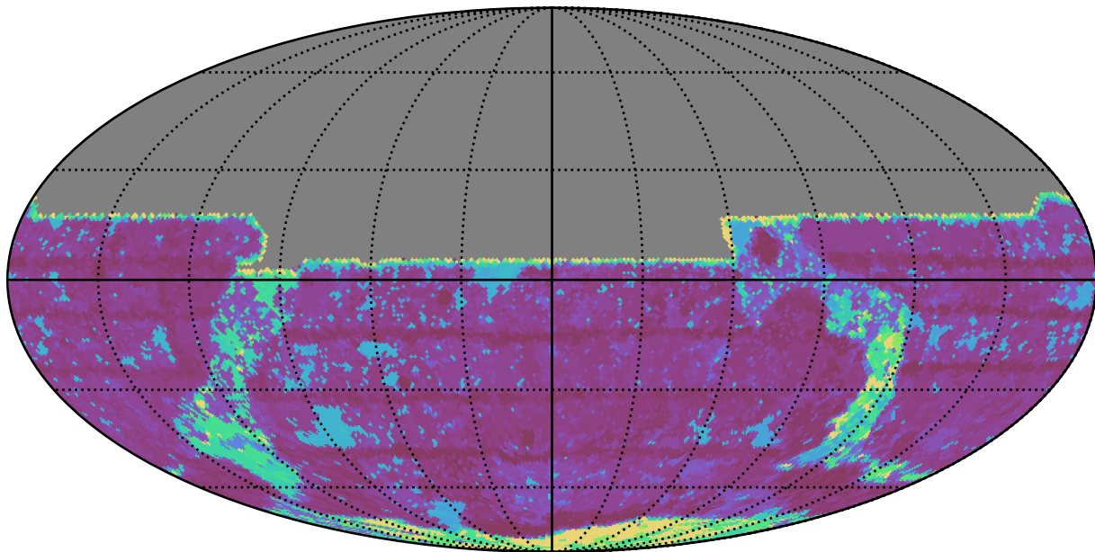
ddf_acor_sf10_lsf30_lsr50_v3.4_10yrs All sky y band: Max Inter-Night Gap
